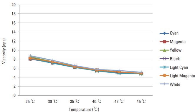
VISCOSITY DATA
